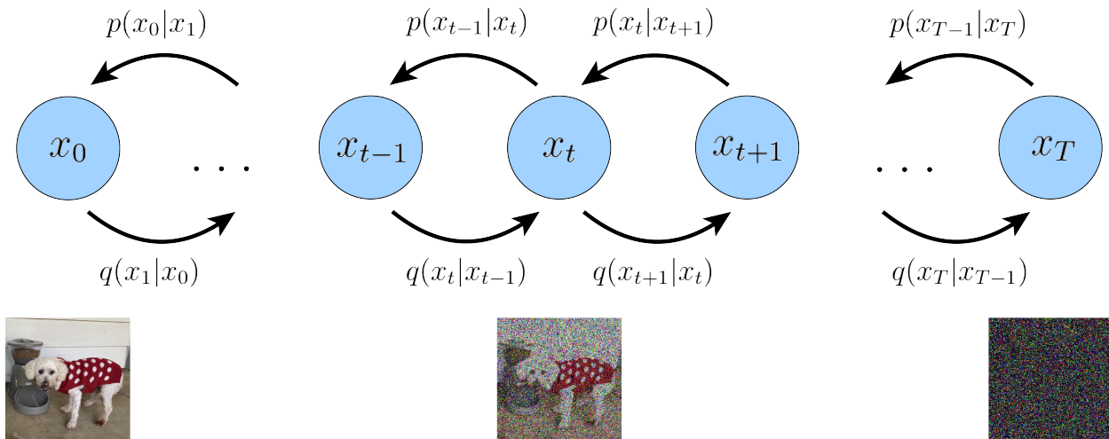
Figure 3: A visual representation of a Variational Diffusion Model; \mathbf{x}_0 represents true data observations such as natural images, \mathbf{x}_T represents pure Gaussian noise, and \mathbf{x}_t is an intermediate noisy version of \mathbf{x}_0 . Each q(\mathbf{x}_t|\mathbf{x}_{t-1}) is modeled as a Gaussian distribution that uses the output of the previous state as its mean.
