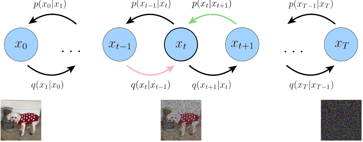
Figure 4: Under our first derivation, a VDM can be optimized by ensuring that for every intermediate \mathbf{x}_t , the posterior from the latent above it p_\theta(\mathbf{x}_t|\mathbf{x}_{t+1}) matches the Gaussian corruption of the latent before it q(\mathbf{x}_t|\mathbf{x}_{t-1}) . In this figure, for each intermediate \mathbf{x}_t , we minimize the difference between the distributions represented by the pink and green arrows.
