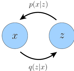
Figure 1: A Variational Autoencoder graphically represented. Here, encoder q(\mathbf{z}|\mathbf{x}) defines a distribution over latent variables \mathbf{z} for observations \mathbf{x} , and p(\mathbf{x}|\mathbf{z}) decodes latent variables into observations.
